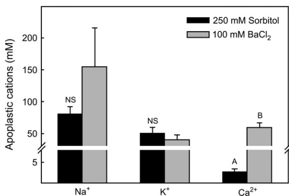
Fig. 2. Concentration of soluble (250 mM sorbitol infiltration solution) and exchangeable plus soluble (100 mM BaCl 2 infiltration solution) Na + , K + , and Ca 2+ in the leaf apoplast of Sarcobatus (mean \pm SE, n=44-86 ). Values for the two different infiltration solutions were averaged across the four salinity treatments. Letters indicate significant differences in cation concentration ( P < 0.05 ) between infiltration solutions. Note scale change across y-axis break.
