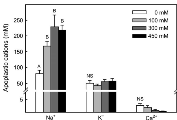
Fig. 1. Concentration of soluble Na + , K + , and Ca 2+ in the leaf apoplast of Sarcobatus growing in four salinity treatments (mean \pm SE, n=30-55 ). Each replicate measurement was made on approximately 4 g FW of leaves infiltrated with 250 mM sorbitol and centrifuged at 600 g for 6 min. Letters indicate significant differences in cation concentration ( P < 0.05 ) between salinity treatments. Note scale change across y-axis break.
